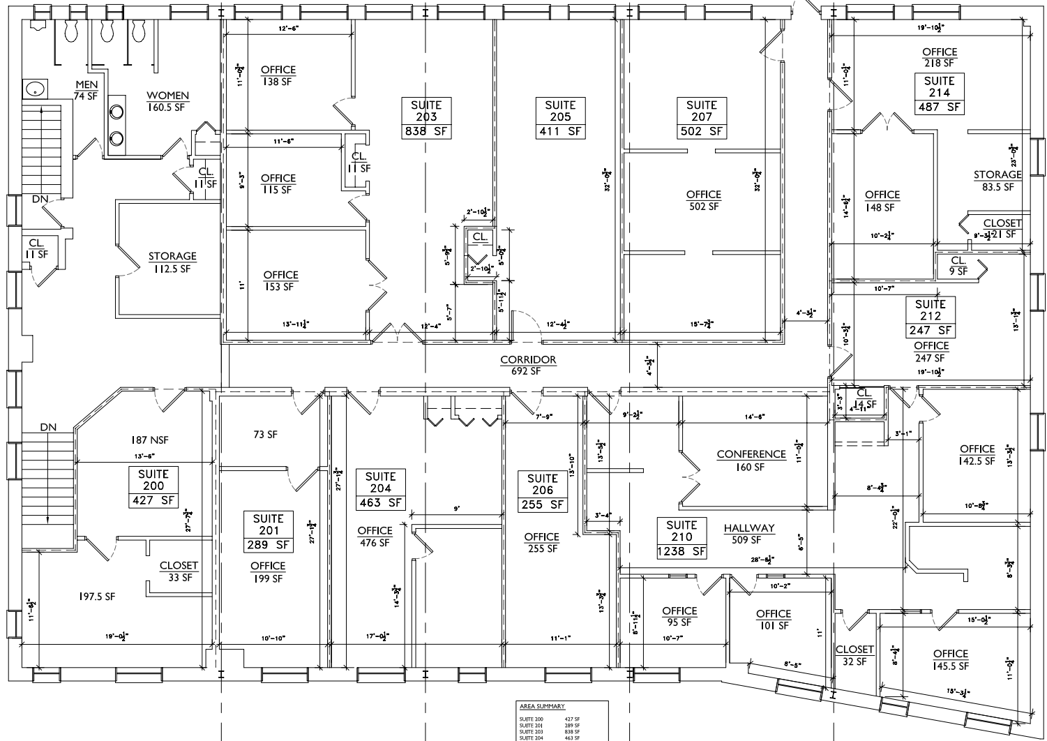
(E5) SECOND FLOOR PLAN NOT TO SCALE
